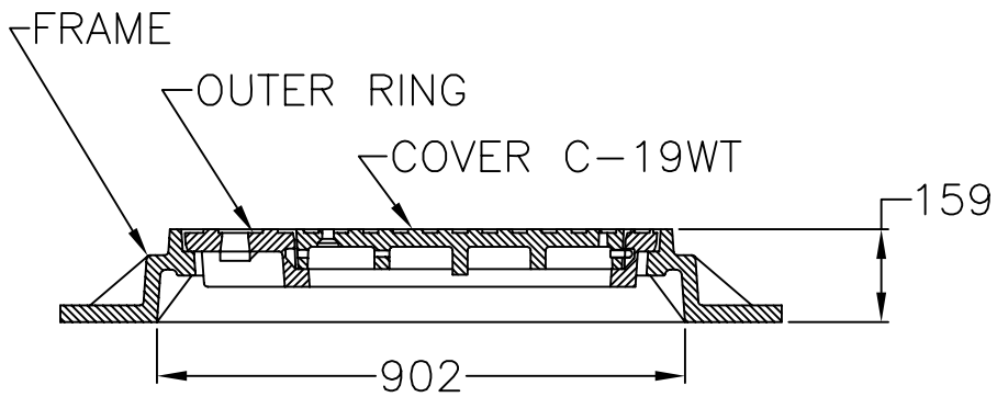
SECTION OF FRAME, RING AND COVER.
